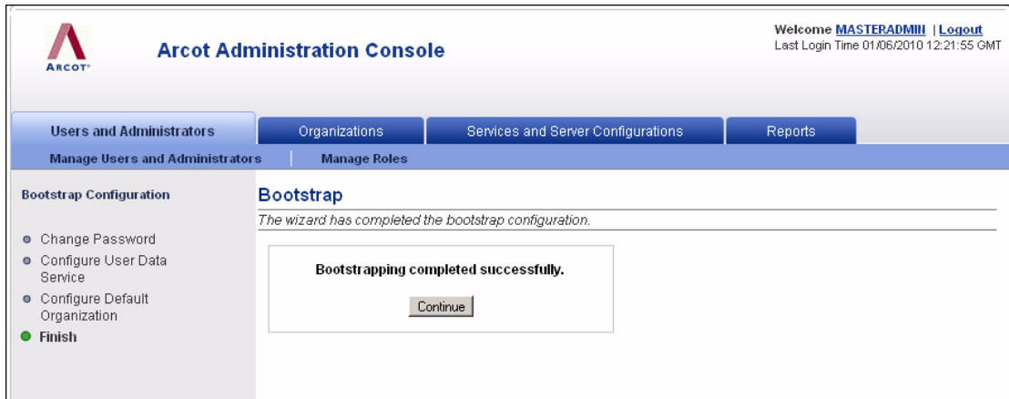
Figure 5-5 Bootstrap Wizard: Finish Screen
