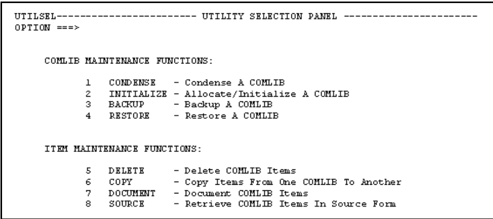
Figure 2-51 The Utility Selection Menu Panel
