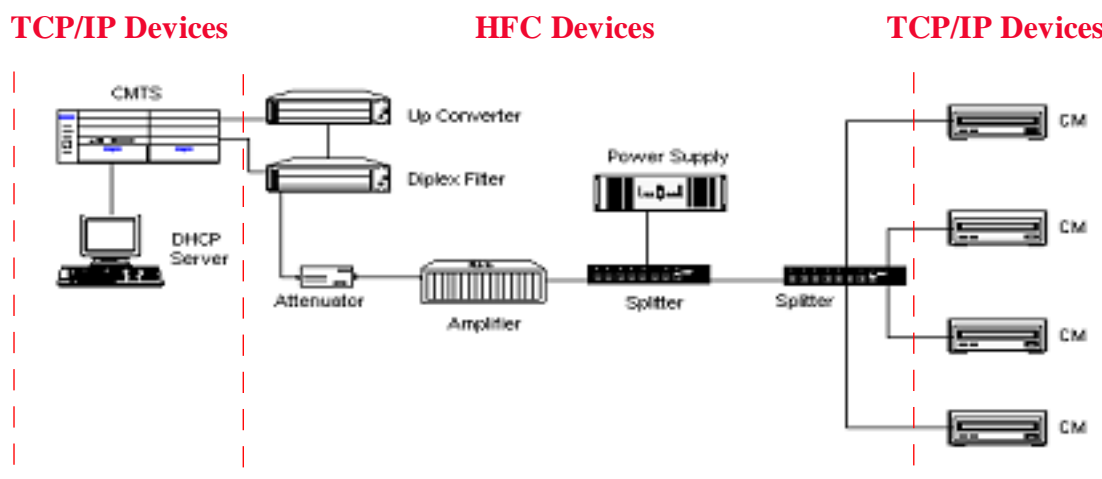
Basic Components of a Cable Broadband Network
