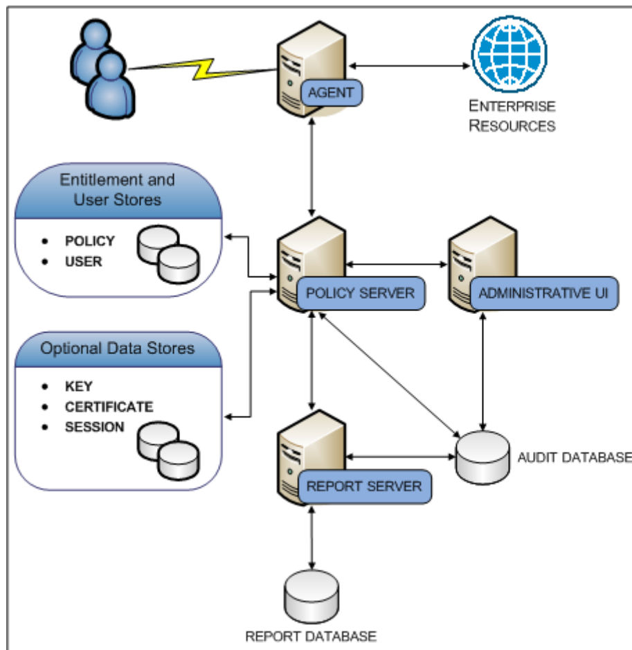
Figure 2: Simple deployment with optional components
