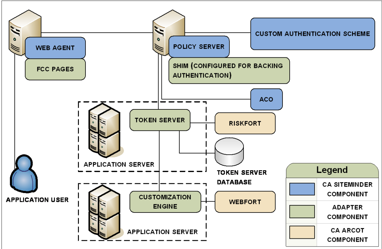
Figure 5: CA SiteMinder authentication and CA Arcot risk analysis
