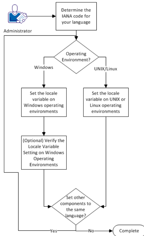
How to Set Log Files, and Command-line Help to Another Language
