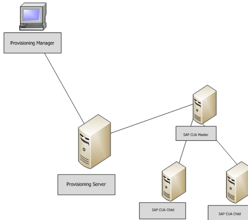
Figure 1: Provisioning Server connects to SAP CUA Master, which connects to any SAP CUA Child system
