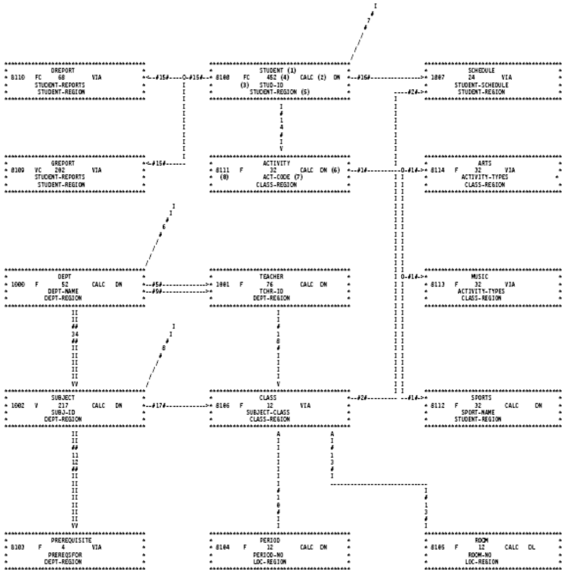
Exhibit 3.1: Sample of a Simple Data Structure Diagram
