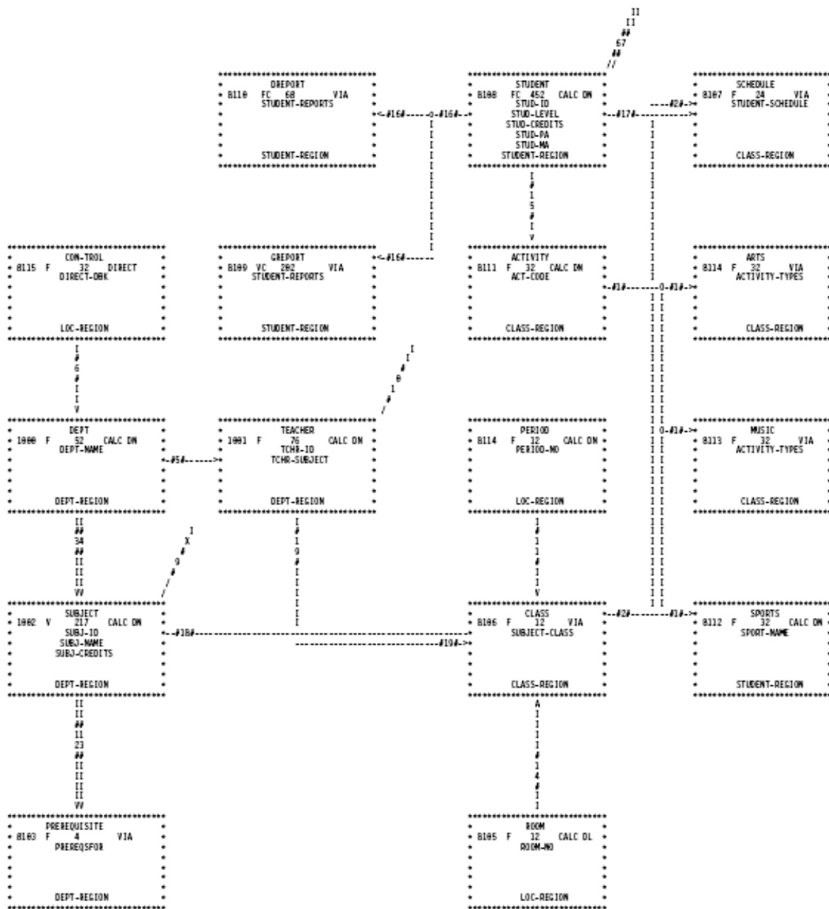
Exhibit 4.14: Default CA IDMS Schema Mapper Data Structure Diagram with Multiple CALC Keys
