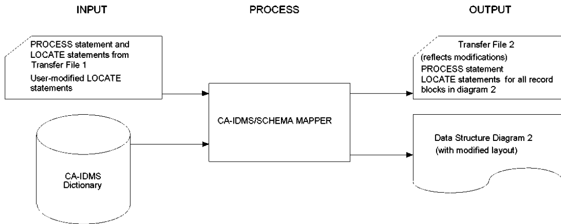
Exhibit 1.5c: Using the Transfer File to Add Record Blocks to the Diagram
