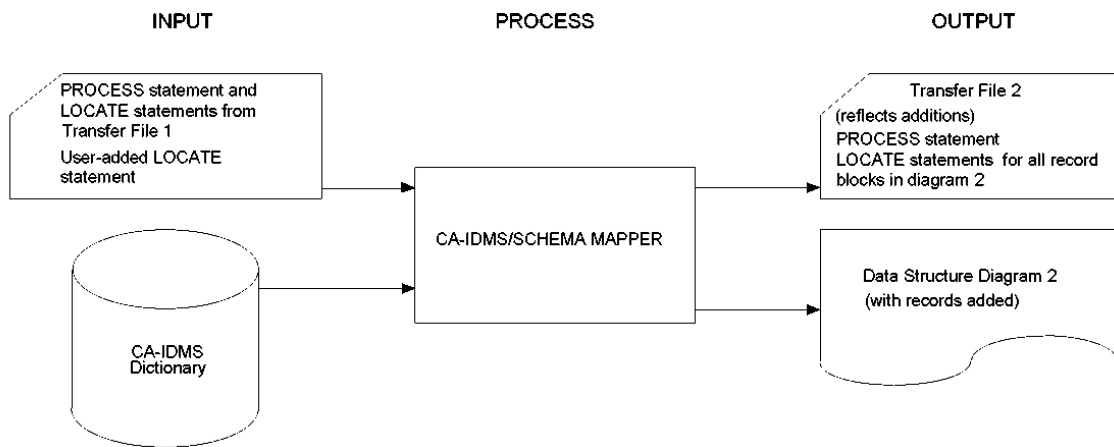
Exhibit 1.5b: Using the Transfer File to Produce the Identical Diagram
