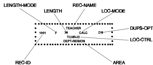
Exhibit 2.4: Default Record Block with Field Names in a Four Line Format
