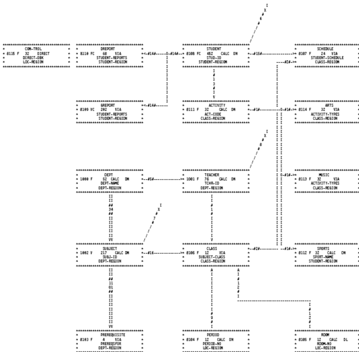
Exhibit 4.4: Default CA IDMS Schema Mapper Data Structure Diagram
