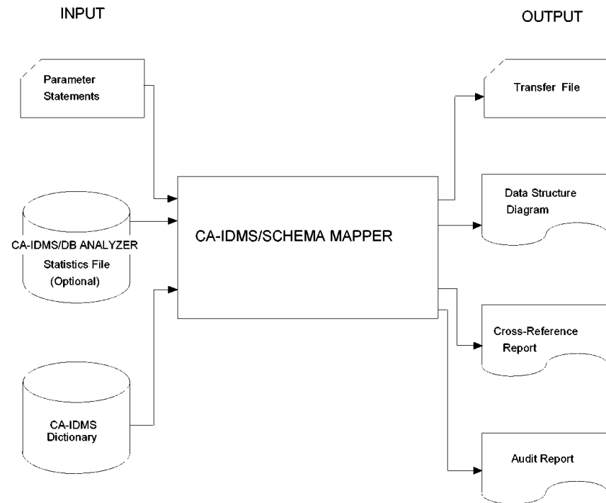
Exhibit 1.1: CA IDMS Schema Mapper Process
