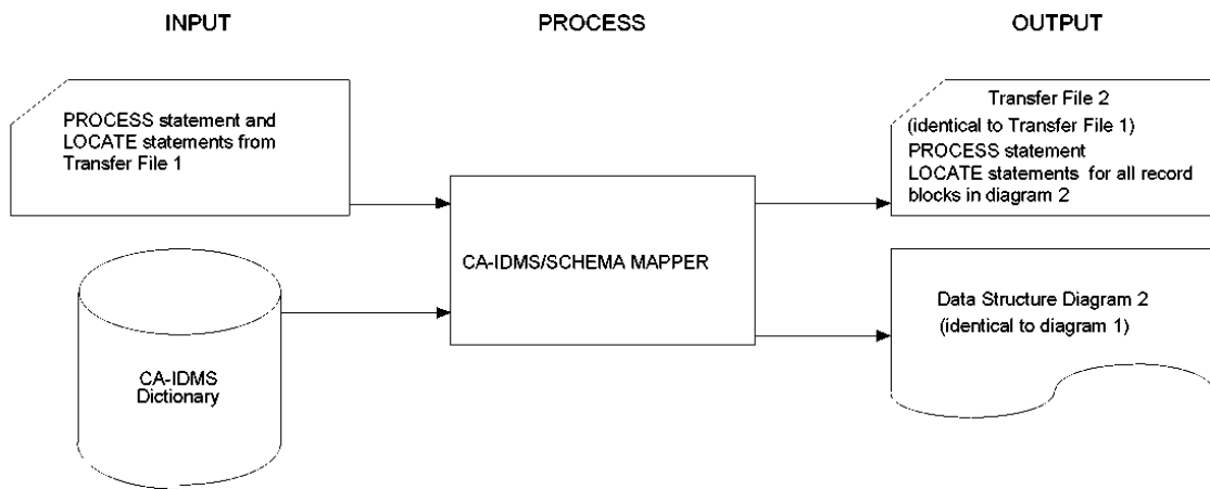
Exhibit 1.5a: Step 1 for Using the Transfer File
