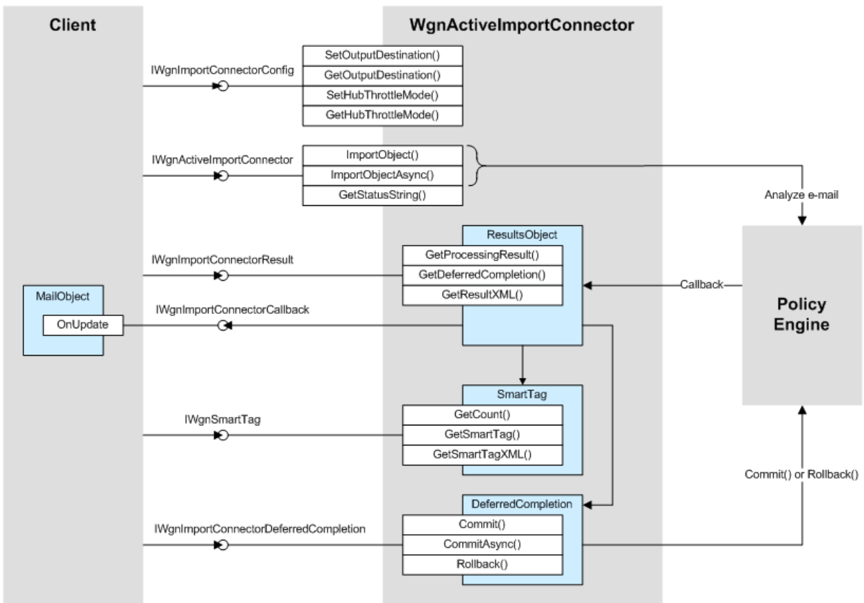
CA DataMinder External Agent: Interfaces and methods()
